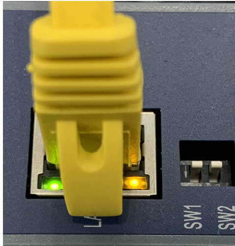
图 4-21: RJ45 LED
